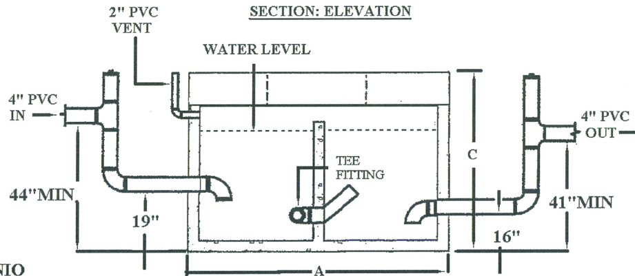
SECTION: ELEVATION
